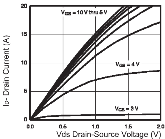
Figure 5 Output Characteristics
