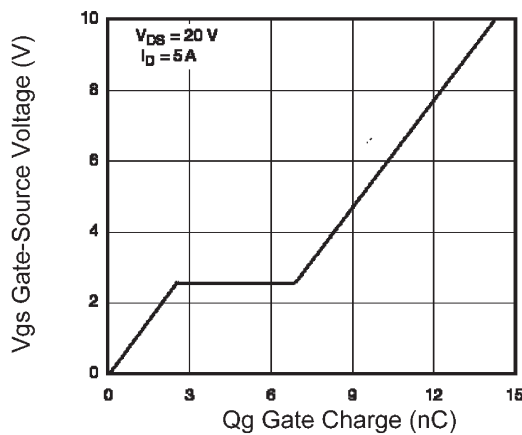
Figure 11 Gate Charge
