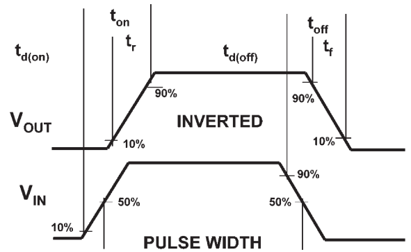
Figure 2: Switching Waveforms
