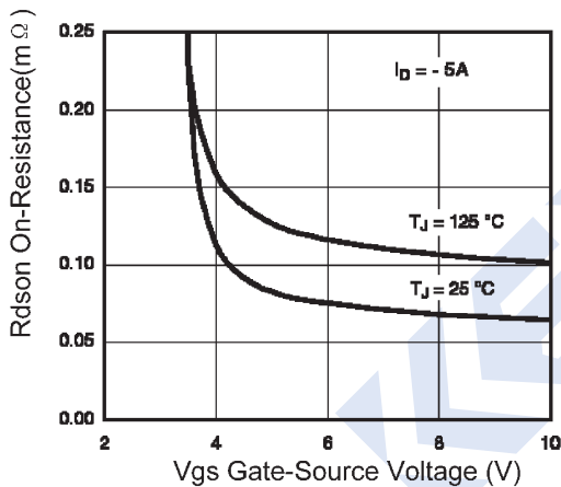
Figure 9 Rdson vs Vgs
