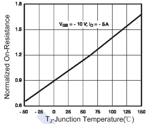
Figure 8 Drain-Source On-Resistance
