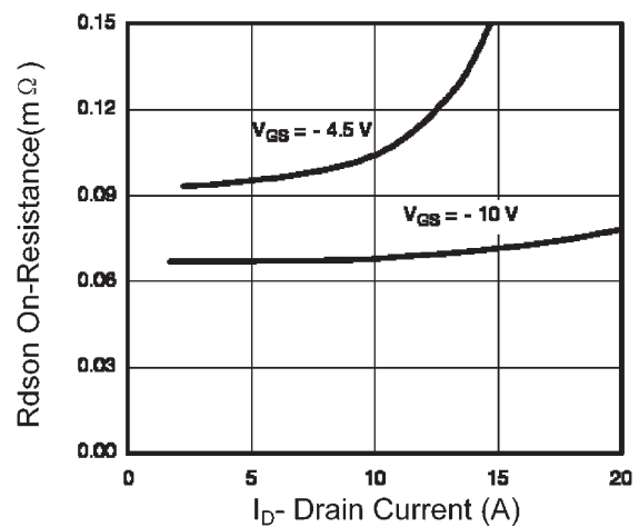
Figure 6 Drain-Source On-Resistance
